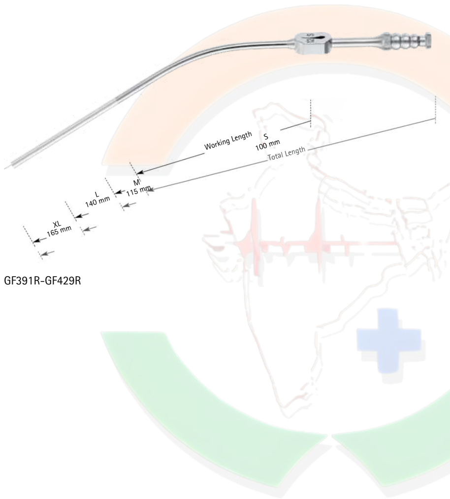
Suction Tube, Fukushima Style, W/ Tapered Teardrop Control
